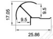
KSD-9515 Weight: 0.079kg/m
