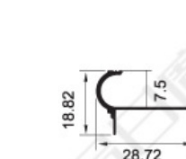
KST-FP107 Weight: 0.131kg/m
