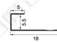
KSD-ZH1061A Weight:0.027kg/m
