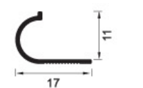
KST-H11.9 Weight: 0.077kg/m
