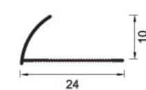
KST-LC20 Weight: 0.063kg/m
