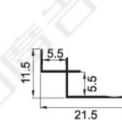
KSD-067 Weight: 0.050kg/m
