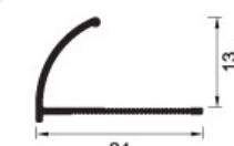
KST-FK125 Weight: 0.106kg/m
