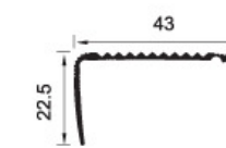
KST-L20B Weight: 0.21kg/m
