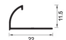
KST-Y9.1 Weight: 0.083kg/m
