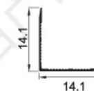
KST-2000-ZH031 Weight: 0.033kg/m
