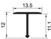
KST-MT13.4 Weight: 0.0585kg/m
