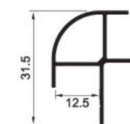
KST12.5 Weight: 0.259kg/m
