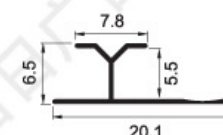
KSD-062 Weight: 0.043kg/m
