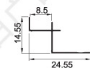
KSD-8603 Weight: 0.054kg/m
