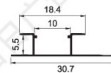
KSD-064 Weight: 0.069kg/m
