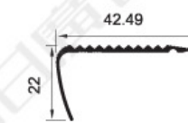
KST-YL22 Weight: 0.21kg/m
