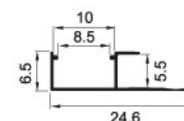
KSD-065 Weight:0.056kg/m
