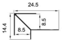
KSD-8502 Weight: 0.064kg/m
