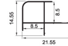
KSD-8609 Weight: 0.071kg/m
