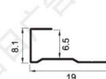
KSD-6504 Weight:0.039kg/m
