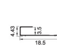
KSD-D179 Weight:0.029kg/m
