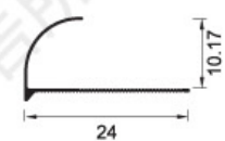
KST-K10C1 Weight: 0.048kg/m
