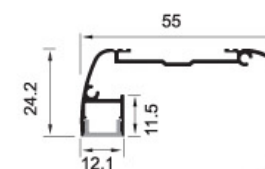
KST-CJTK55LED Weight: 0.318kg/m
