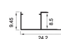
KSD-8511 Weight:0.058kg/m
