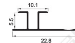
KSD-068 Weight: 0.054kg/m
