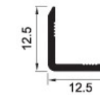
KST-Z12.5X12.5 Weight: 0.083kg/m
