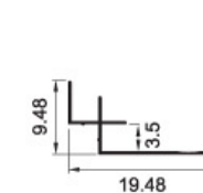
KSD-D178 Weight: 0.036kg/m
