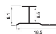
KSD-6501 Weight: 0.038kg/m
