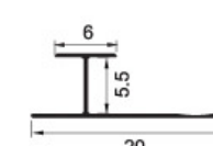
KSD-ZH1060 Weight: 0.032kg/m
