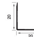
KST-V20 Weight: 0.086kg/m
