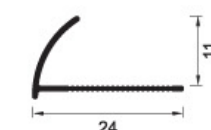
KST-FA105 Weight: 0.093kg/m
