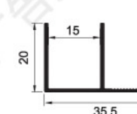
KST-F15X20 Weight:0.216kg/m
