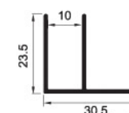
KST-F23.5X10 Weight:0.243kg/m
