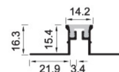
KST-KT15.4 Weight: 0.138kg/m
