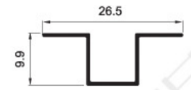
KST-XJ10 Weight: 0.085kg/m
