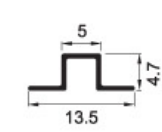
KST-2000-ZH019 Weight: 0.035kg/m
