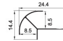
KSD-8515 Weight: 0.051kg/m
