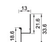
KST-LUZ9.6 Weight:0.1kg/m
