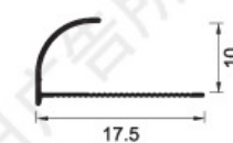
KST-K10B Weight: 0.0734kg/m
