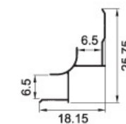
KSD-6503 Weight: 0.06kg/m
