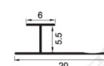
KSD-060 Weight: 0.036kg/m
