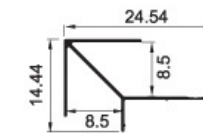
KSD-8602 Weight: 0.072kg/m
