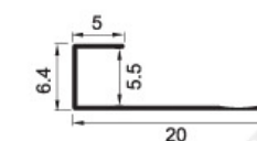
KSD-061 Weight:0.036kg/m
