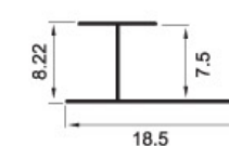
KSD-7419 Weight: 0.033kg/m
