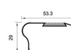
KST-CJTK53.3 Weight: 0.224kg/m
