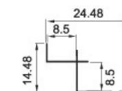
KSD-8503 Weight: 0.046kg/m
