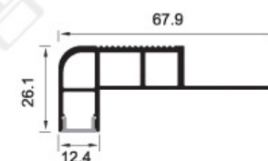
KST-LEDTK12.1 Weight: 0.638kg/m
