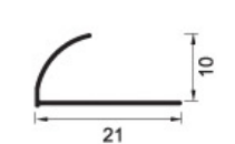
KST-K09 Weight: 0.069kg/m
