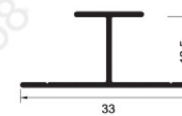
KST12.5 Weight: 0.157kg/m
