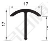
KST-17 Weight: 0.122kg/m
