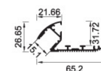
KST-YX65.2 Weight:0.579kg/m
