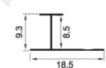
KSD-8501 Weight: 0.035kg/m
