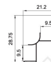
KSD-9503Y Weight: 0.072kg/m
