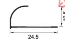
KST-K231 Weight: 0.056kg/m
